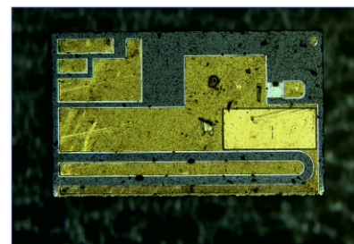
Gold Finger Micro-scratch Detection
